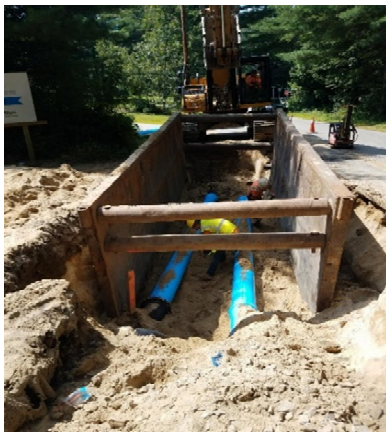
Pipe Installation
