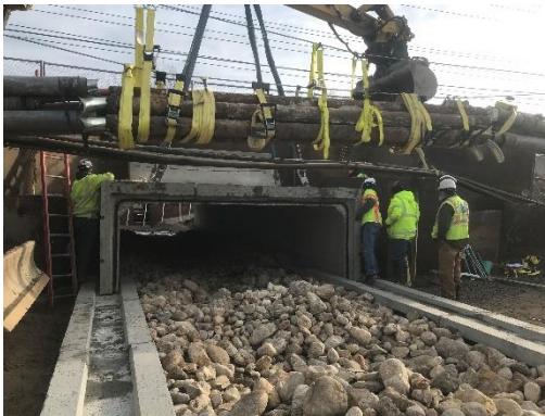
Bridge Section Installation with suspended utilie
