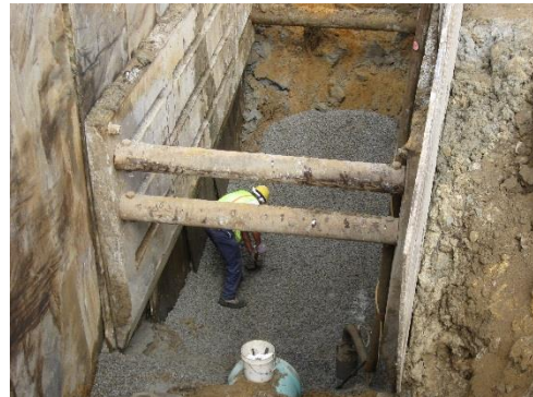
Sewer Main Bedding Installation
