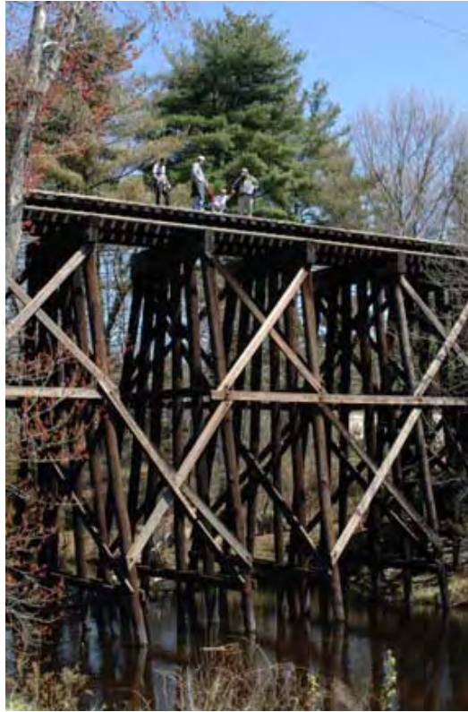
Rail bridge over Great Cojas Brook in Manchester (Photo: John St. Hilaire)
