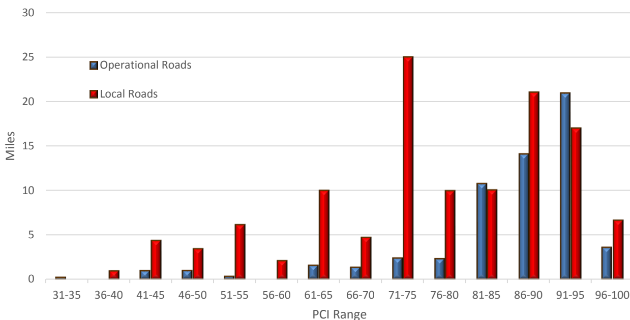
Figure 2 - PCI Distribution- by Functional Classification
