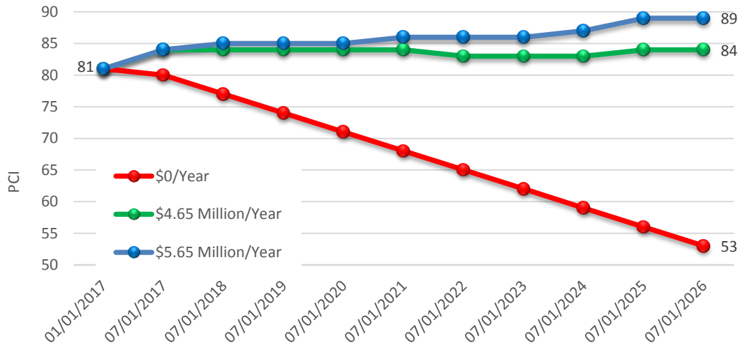
Figure 16 – Projected Pavement Condition
