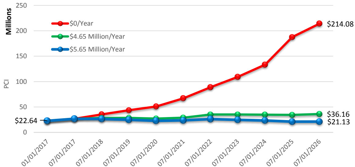
Figure 17 – Projected Backlog Summary
